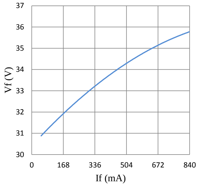
Forward Current vs. Forward Voltage ( T_c=25^{\circ}\text{C} , 6000K)
