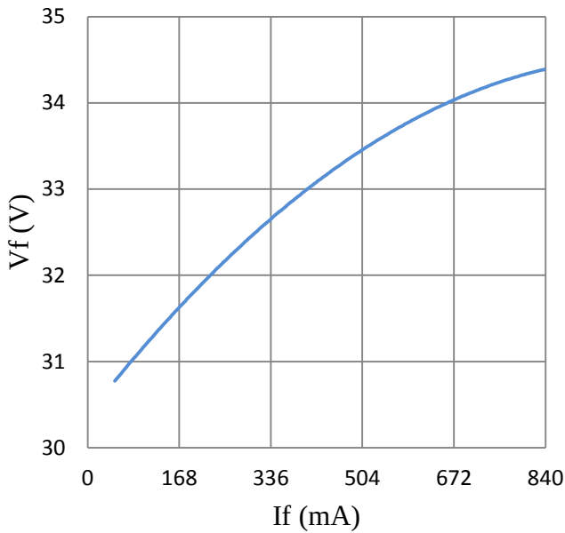
Forward Current vs. Forward Voltage ( T_c=25^{\circ}\text{C} , 2600K)
