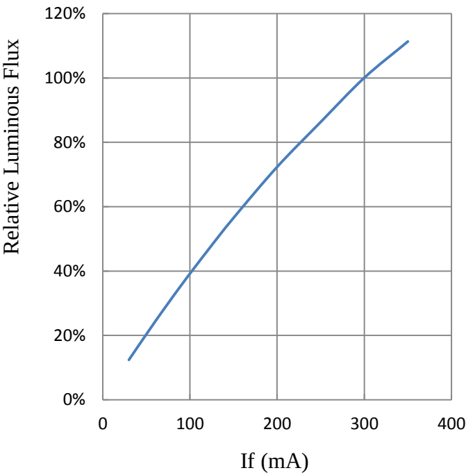
Forward Current vs. Relative Luminous Flux (Tc=25°C )
