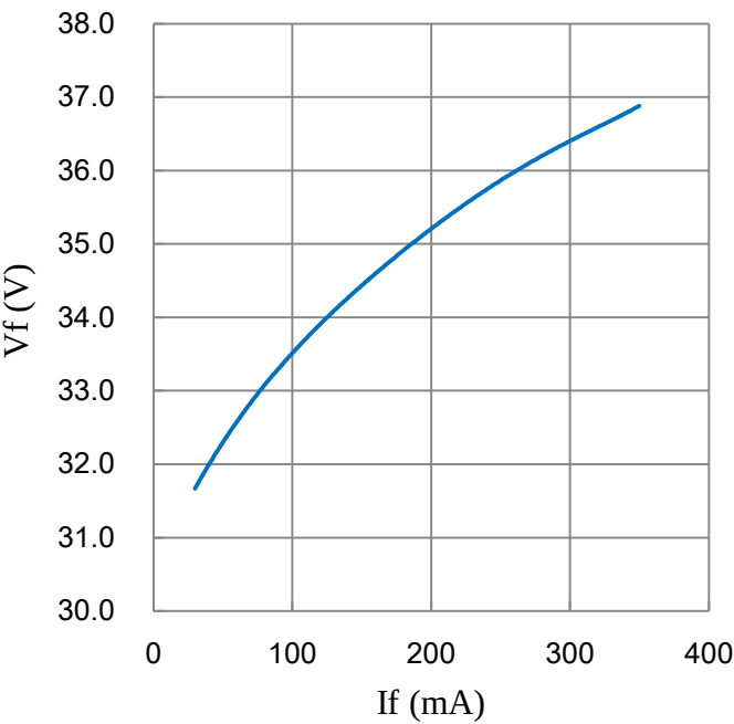
Forward Current vs. Forward Voltage (Tc=25°C )
