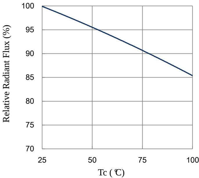
Case Temperature vs. Relative Radiant Flux ( I_f=1920\text{mA} )
