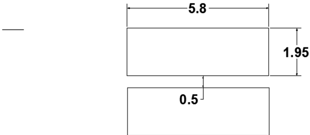
Recommended PCB Soldering Pad Pattern
