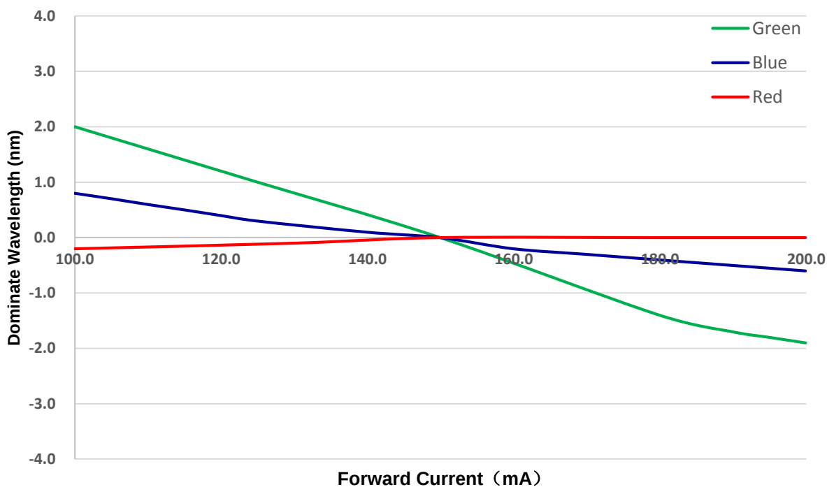
Dominate Wavelength VS Forward Current
