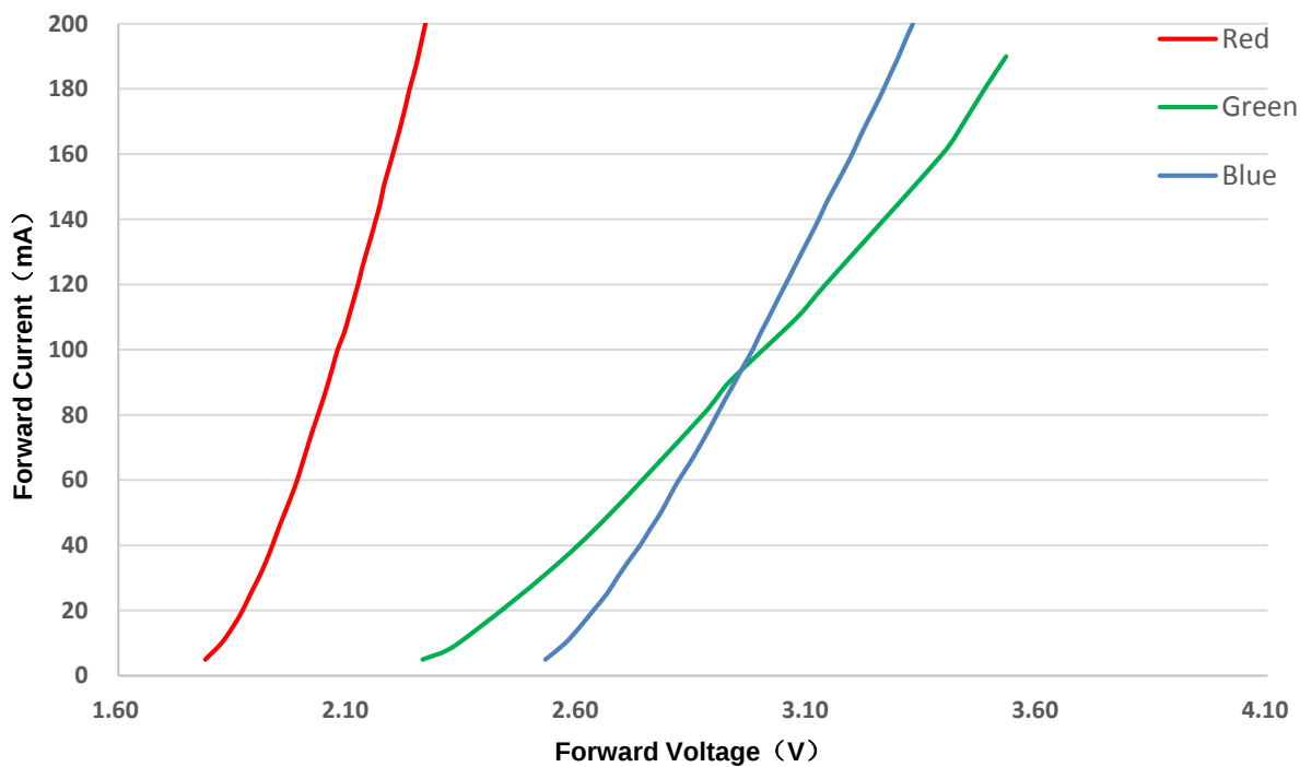
Forward Current VS Forward Voltage
