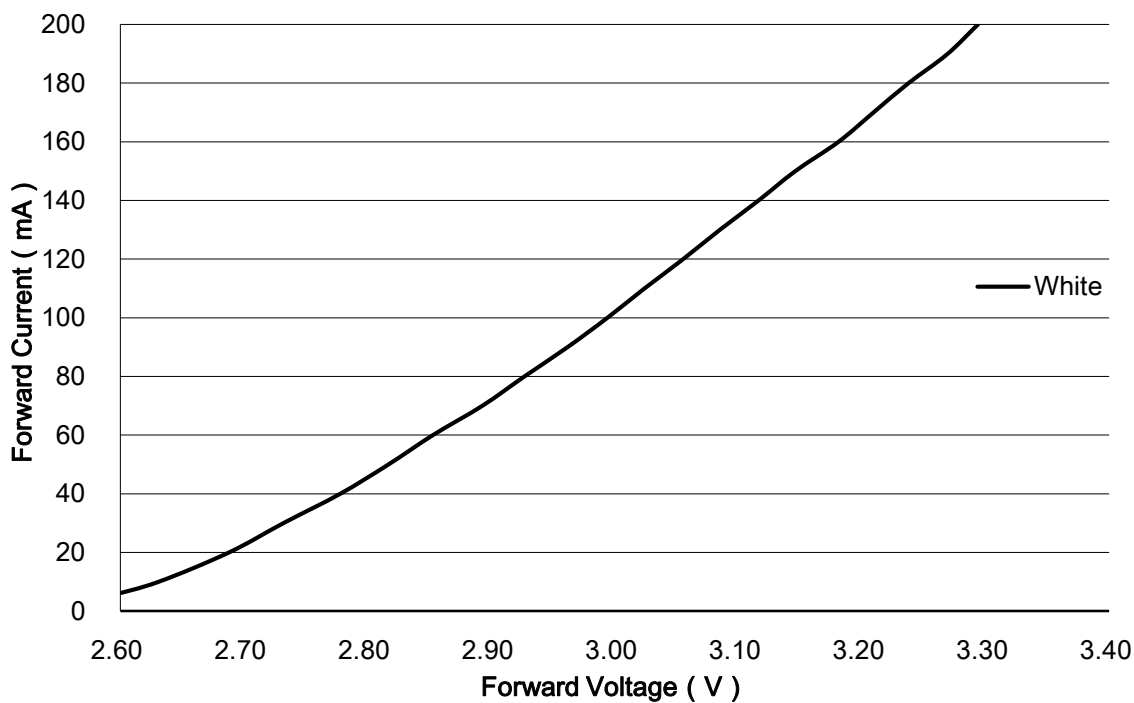
Forward Current vs. Forward Voltage
